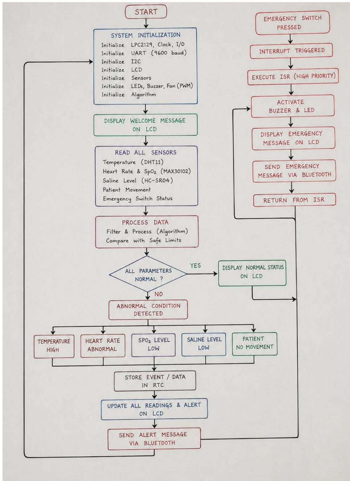
Fig. 3.2 – Working Flow of the Embedded Decision Logic
