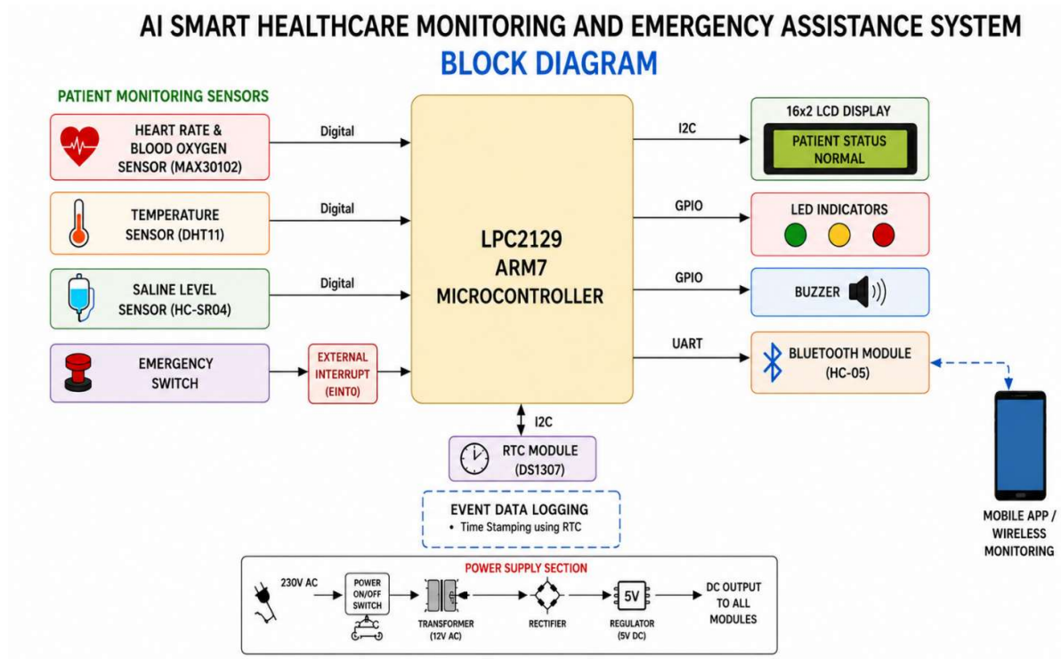
Fig. 3.1 – Block Diagram
